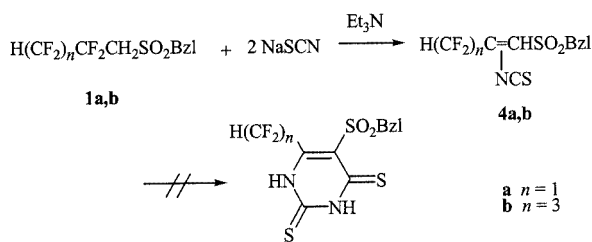
Scheme 3. Reaction between 1 and sodium thiocyanate
