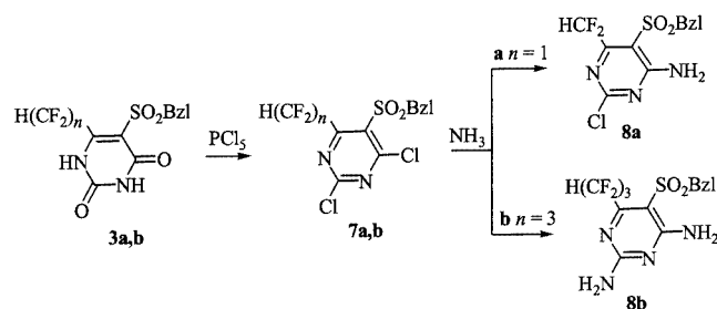
Scheme 5. Synthesis of dichlorides 7a and 7b and their reactions with ammonia
