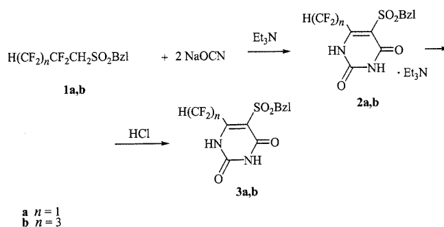
Scheme 1. Synthesis of compounds 3a and 3b
