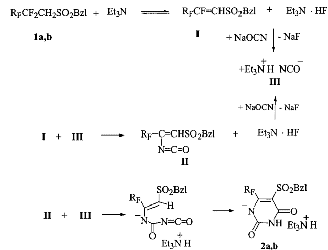
Scheme 2. Proposed reaction sequence for the formation of salts 2a and 2b
