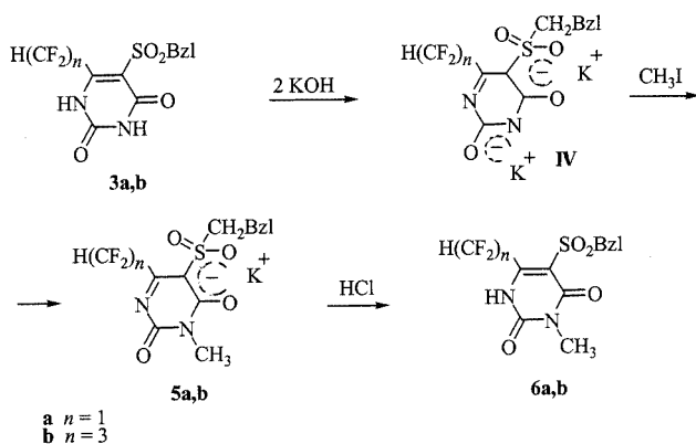
Scheme 4. Alkylation of compounds 3a , 3b with CH 3 I
