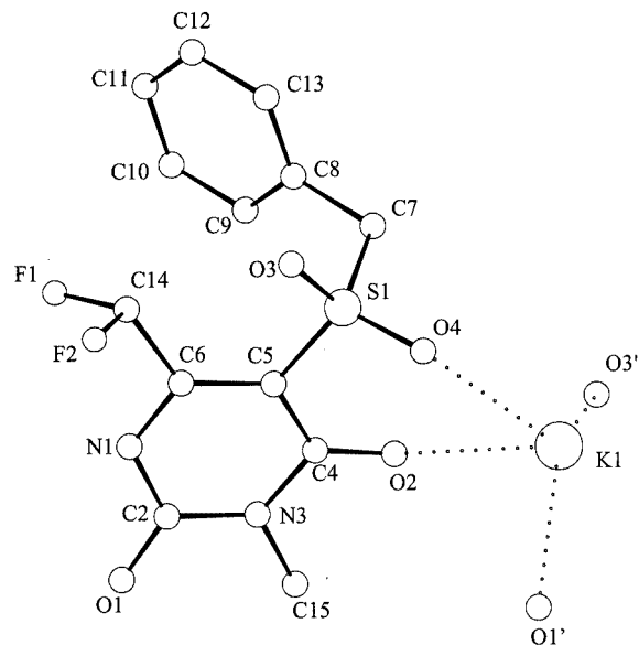
Figure 2. Crystal structure of the salt 5a ; selected interatomic distances [Å] and angles [°]: K(1)⋯O(2) 2.624(2), K(1)⋯O(4) 2.885(2), K(1)⋯O(1') 2.763(2), K(1)⋯O(3'') 2.799(2) Å, O(2)K(1)O(4) 61.4(2)° [primed and double primed atoms are connected with the corresponding atoms in the asymmetric unit by the (− x + 2, − y , − z + 2) and ( x − 3/2, − y − 1/2, z − 1/2) operations]; hydrogen atoms are omitted for clarity
