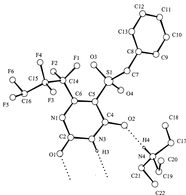
Figure 1. Crystal structure of the salt 2b ; selected interatomic distances [Å] and angles [°]: N(4)···O(2) 2.791(2), H(4)···O(2) 1.93(3) Å, N(4)H(4)O(2) 173(2)°; N(3)···O(1') 2.776(2), H(3)···O(1') 1.95(3) Å, N(3)H(3)O(1') 174(2)° (primed atoms are generated from the asymmetric unit by the inversion center)
