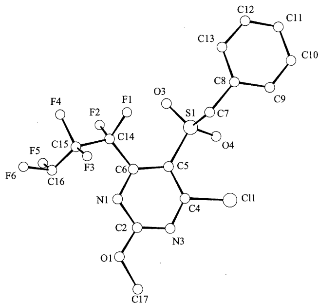
Figure 4. A perspective view and labelling scheme for the independent molecule A of the compound 9b ; hydrogen atoms are omitted for clarity
