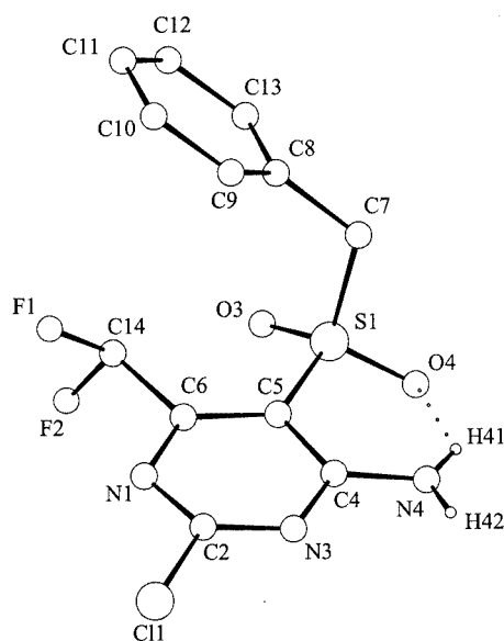
Figure 3. A perspective view and labelling scheme for the molecule 8a ; the main geometrical parameters of the intramolecular H bond: N(4)···O(4) 2.722(3), O(4)···H(41) 2.02(3) Å, N(4)H(41)O(4) 135.2(2)°
