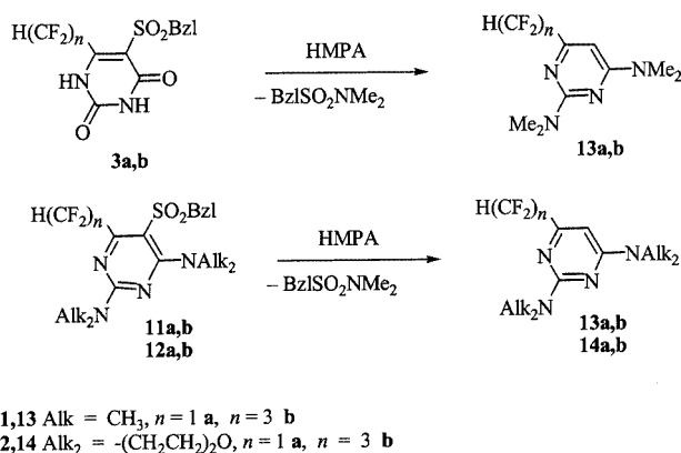
Scheme 8. Desulfonylation of compounds 3 , 11 , and 12
